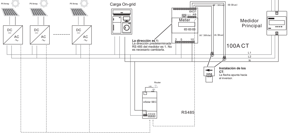
RS485
