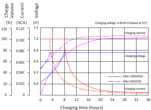
Charging characteristics
