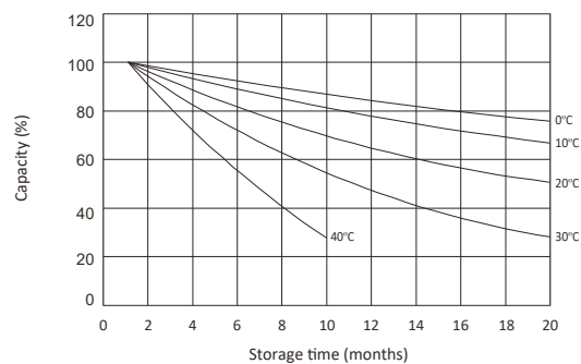
Temperature effect on battery self-discharge
